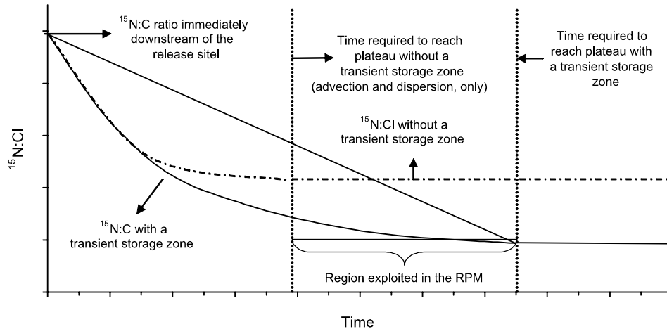
Fig. 2. A theoretical example of the change in \text{NO}_3\text{-}^{15}\text{N}:\text{Cl} ratio ( R ) through time at a location some distance downstream of an experimental solute addition point. The dashed and solid lines illustrate the expected temporal pattern in R in the absence and presence of a transient storage zone, respectively.
