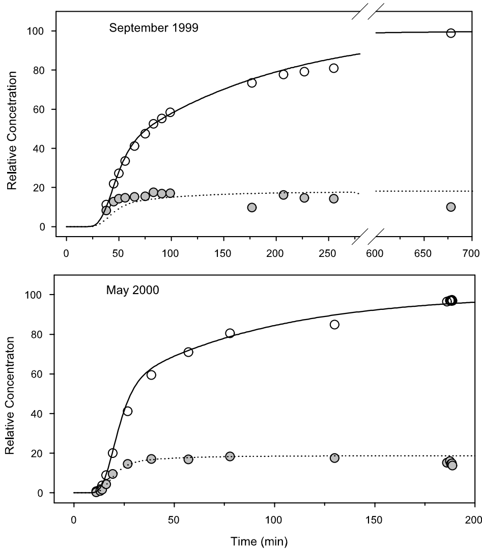
Fig. 4. The relationship between the field data and predicted values using a one-dimensional transport model with transient storage and reactive uptake. The uptake coefficients are first-order rate constants ( \lambda and \lambda_S ) derived from the Regression Partitioning Method.
