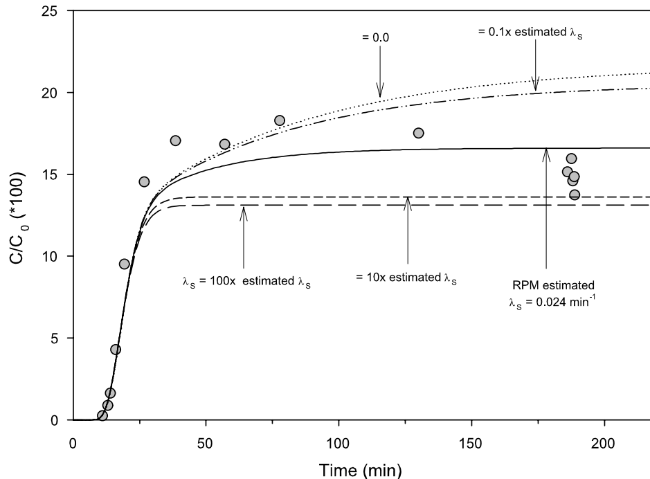
Fig. 5. The sensitivity of reactive transport model to variation in \lambda_s , May 2000.
