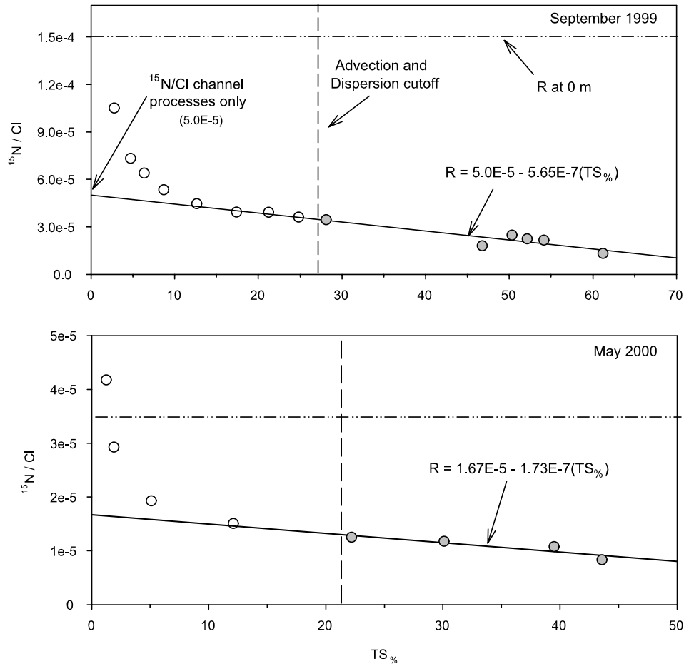
Fig. 3. Regressions between the ratio of reactive to conservative solute ( \text{NO}_3\text{-}^{15}\text{N}:\text{Cl} ) and the percentage of water that has resided within the transient storage zone ( \text{TS}\% ). All regressions were significant ( p < 0.05 ).
